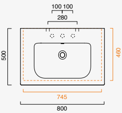
Sfera 80x50 cod. 180SFN00
