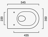
Sfera Wc Newflush 54x35 cod. 1VSF54R00
