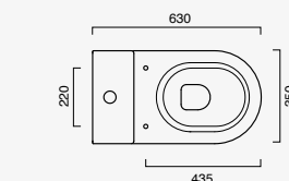
Sfera Wc Monoblocco 63x35 cod. 1MPSFN00 + 1CMSZ00
