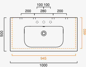
Sfera 100x50 cod. 1100SFN00
