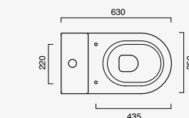
Sfera Wc Monoblocco 63x35 cod. 1MPSFN00 + 1SCSC00
