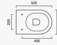
Sfera Wc 52x35 cod. 1VPC5200
