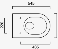
Sfera Wc Eco Newflush 54x35 cod. 1VSF54RECO00
