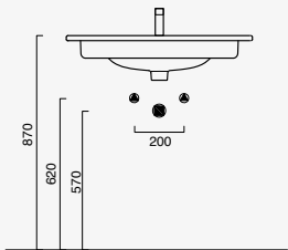
Sfera 60x45 cod. 160BSF00
