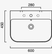
Sfera 60x45 cod. 160BSF00
