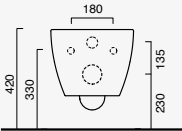
Sfera Wc Eco Newflush 54x35 cod. 1VSF54RECO00
