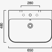
Sfera 65x48 cod. 165BSF00
