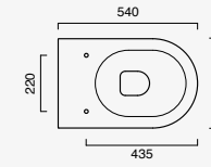
Sfera Wc 54x35 cod. 1VPS5400
