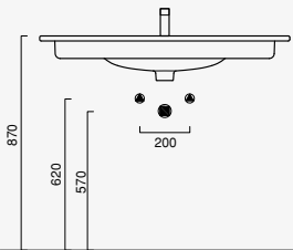
Sfera 65x48 cod. 165BSF00
