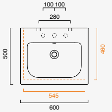
Sfera 60x50 cod. 160SFN00
