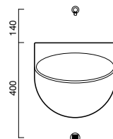
RUBINETTO A PARETE WALL-HUNG TAP WANDARMATUREN
