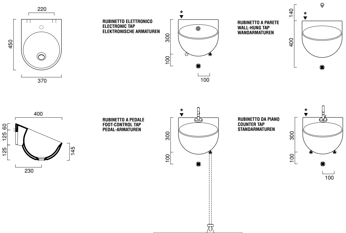
Sistema GIRLY - LAVAMANI HANDLY / HANDWASHBASIN HANDLY / WASCHTISCH HANDLY - HANDLY - Kg. 12
