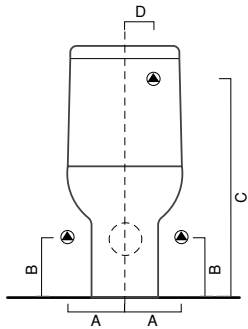
Sistema SFERA - WC MONOBLOCCO / CLOSE-COUPLED WC / STAND KOMBINATION WC - MPSN - Kg. 22
