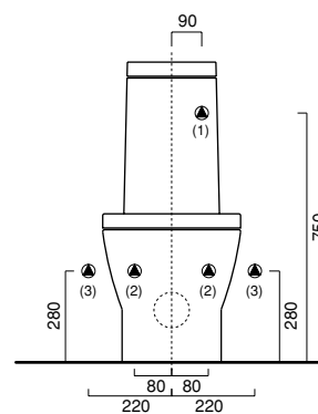
Sistema ZERO+ - WC 58 MONOBLOCCO / CLOSE-COUPLED WC 58 / STAND KOMBINATION WC 58 - MPZG - Kg. 25 dwg ● dxf ●
